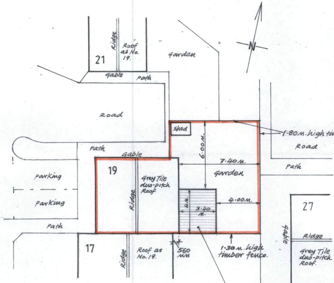
SITE/ROOF PLAN 1:200
